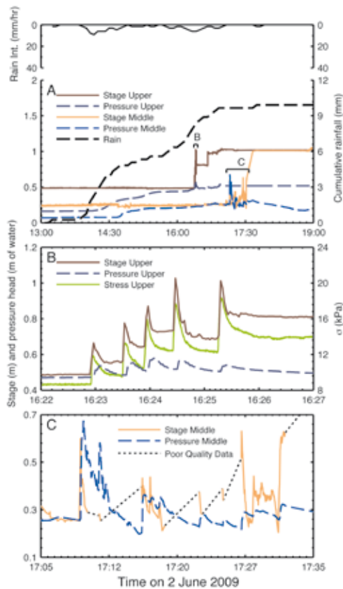
Fig. 3 - Sensor data 2 June 2009. A) Upper axis: 10-minute rainfall intensities measured at the upper station. Lower axis: Complete event duration measured at the upper and middle station. Flows stopped upstream of the lower station. The first debris flows initiated in the west channel, arrived at the upper station at 16:22:54 and stopped before reaching the middle station. The second set of debris flows initiated in the east channel and arrived at the middle station at 17:09:14. Pre-flow sediment depth at the upper station was 0.47 m and 0.26 m at the middle station. Net change in sediment depth was +0.54 m and +0.78 m at the upper and middle station, respectively. Due to rain at 11:00, pre-event pore pressures were not zero. B) 5-minute time slice encompassing the arrival of the first 5 debris-flow surges at the upper station. C) 20-minute time slice from the middle station
