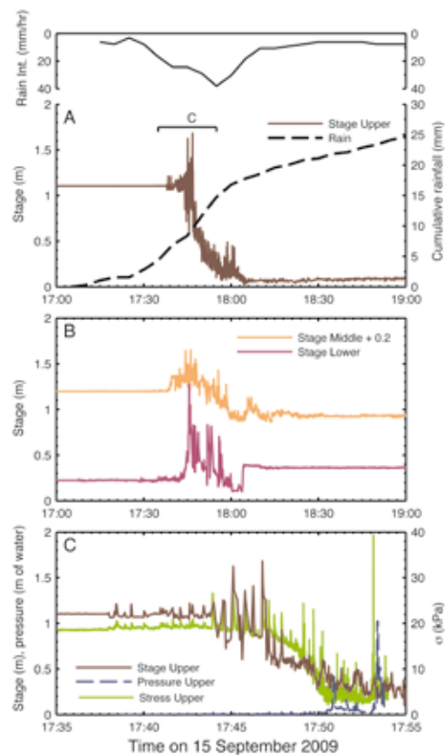
Fig. 6 - Sensor data 15 September 2009. A) Upper axis: 10-minute rainfall intensities measured at the upper station. Lower axis: Complete event duration measured at the upper station. B) Complete event duration measured at the middle and lower stations. Stage at middle station shifted +0.2 m. The first surge front reached the upper, middle and lower stations at 17:38:18, 17:38:40, and 17:42:41, respectively. Pre-flow sediment depths at the upper, middle and lower stations were 1.1 m, 1.0 m, and 0.22 m, respectively. Net changes in sediment depth at the upper, middle and lower stations were -1.1 m, -0.28 m, and +0.14 m, respectively C): 20-minute time slice from the upper station
