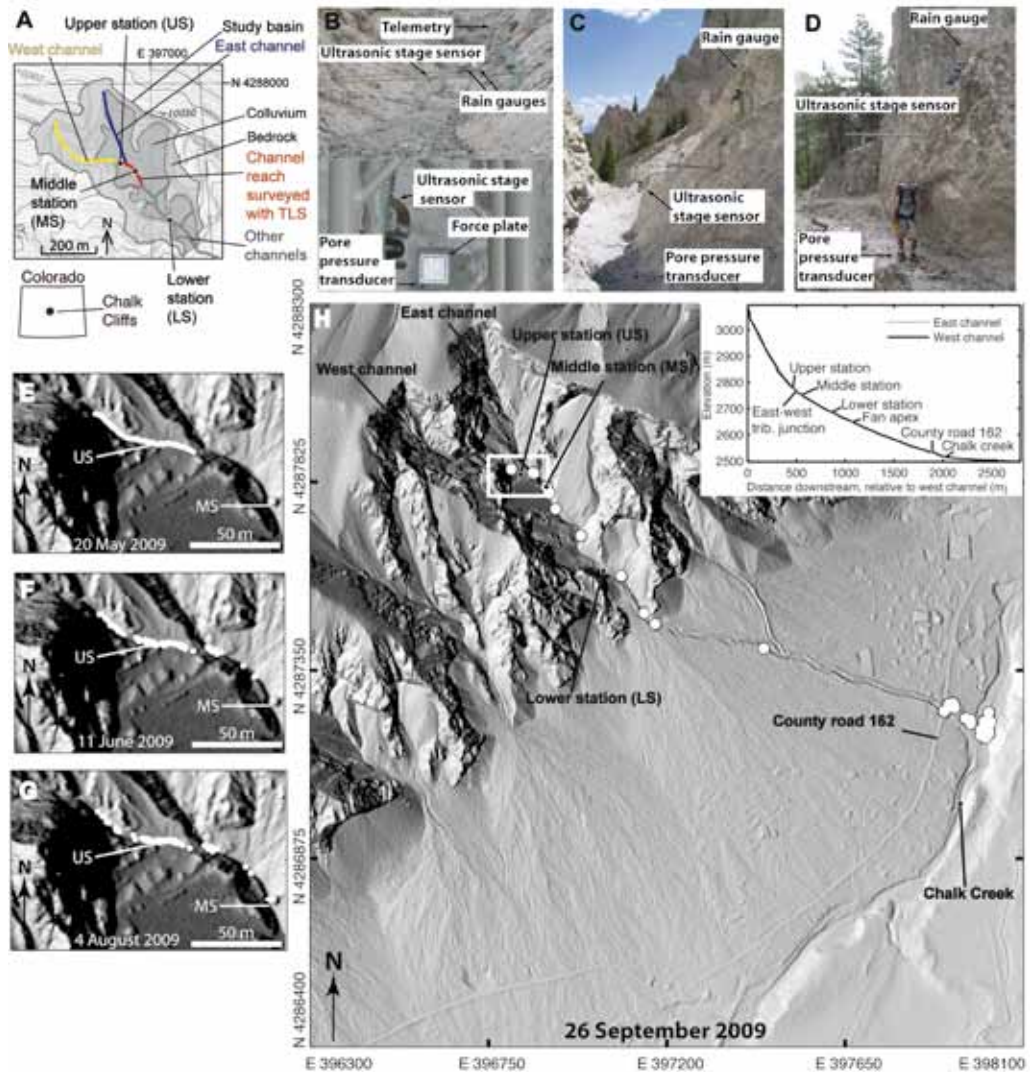
Fig. 1 - Chalk Cliffs study area with photographs of the monitoring stations and shaded relief images (from 1 m ALSM data provided by NCALM) with tracer-particle positions marked by white circles. White rectangle in H encompasses zoomed-in view shown in E, F, and G. A) Line drawing of study basin showing station locations and the distribution of bedrock and colluvium (redrawn from McCoy et alii, 2010) B) Upper station with sensors. C) Middle station. D) Lower station. E) Starting tracer-particle positions 20 May 2009. F) Positions 11 June 2009, 9 days after 2 June 2009 event. G) Positions 4 August 2009, 9 days after 26 July 2009 event. H) Positions 26 September 2009, 11 days after 15 September 2009 event (note no survey was completed after the 06 September 2009 event). Inset: Long profile of east and west channel
