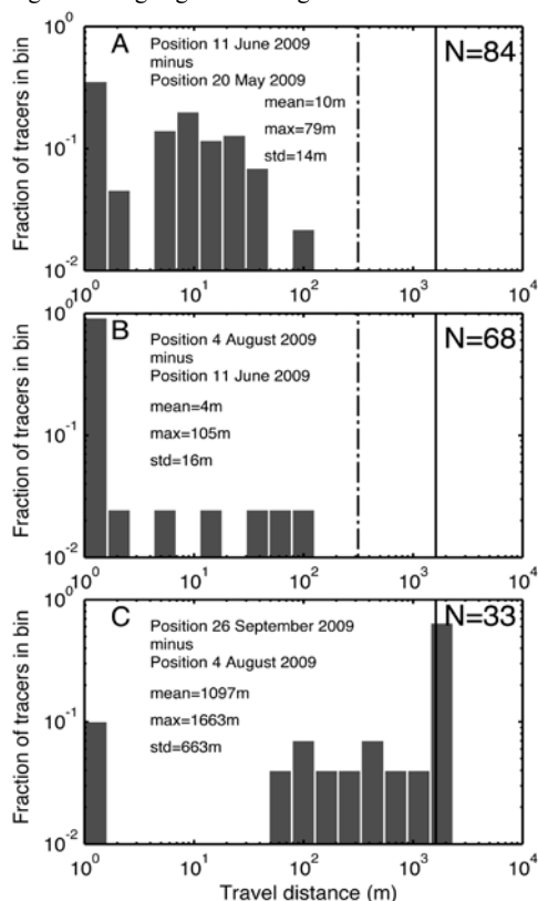
Fig. 2 - Histograms of tracer-particle travel distance between consecutive surveys. Solid line is the travel distance from the mean starting position on 20 May to the junction with the perennial stream Chalk Creek. Dashed line is the distance travelled by the flow front. In C, both lines overlap. A) Distance travelled due to 2 June 2009 event. B) Distance travelled due to 26 July 2009 event. C) Distance travelled due to combination of 6 September 2009 and 15 September 2009 events
