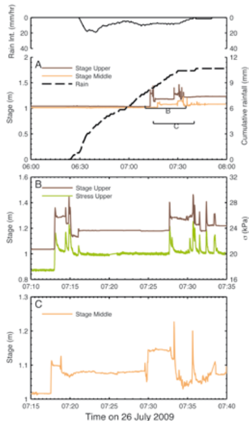
Fig. 4 - Sensor data 26 July 2009. A) Upper axis: 10-minute rainfall intensities measured at the upper station. Lower axis: Complete event duration measured at the upper and middle station. Flows stopped upstream of the lower station. The first surge front reached the upper station at 7:12:42 and the middle station at 7:17:32. Pre-flow sediment depths at the upper and middle stations were 1.04 m, and 1.01 m, respectively. Net changes in sediment depth at the upper and middle stations were +0.19 and +0.07 m, respectively. B) 25-minute time slice from the upper station. C) 25-minute time slice from the middle station
