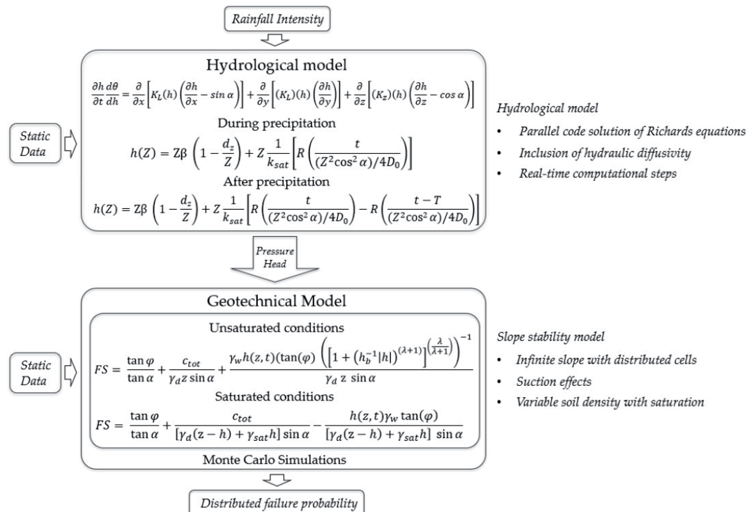
Fig. 2 - Hiresss model structure and main characteristics. Hydrological model: h is the groundwater pressure head, \theta is the soil water volumetric content, t is time, \alpha is the slope angle, K_L and K_z are respectively the hydraulic conductivity in the lateral directions ( x and y ) and the hydraulic conductivity in slope-normal direction ( z ), D_0 is the maximum diffusivity, \beta is a factor depending on rainfall intensity rate (considering Darcy's law for vertical flow in response to infiltration) and K_z d_z is the steady water table, T is the rainfall duration and R is the response function. Geotechnical model: F_s is factor of safety, \phi is the friction angle, \alpha the slope angle, \gamma_d the dry soil unit weight, \gamma_w the water unit weight, h the pressure head, h_b is the bubbling pressure and \lambda the pore size index distribution and \gamma_{sat} is the saturated soil unit weight
