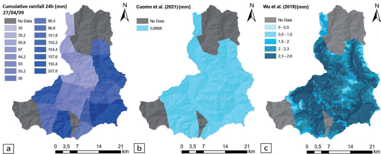
Fig. 3 - Comparison of (a) 24h cumulative rainfall on 27/04/09; (b) 24h rainfall interception by canopies computed with CUOMO et alii (2021); (c) 24h rainfall interception by canopies computed with WU et alii (2019)
