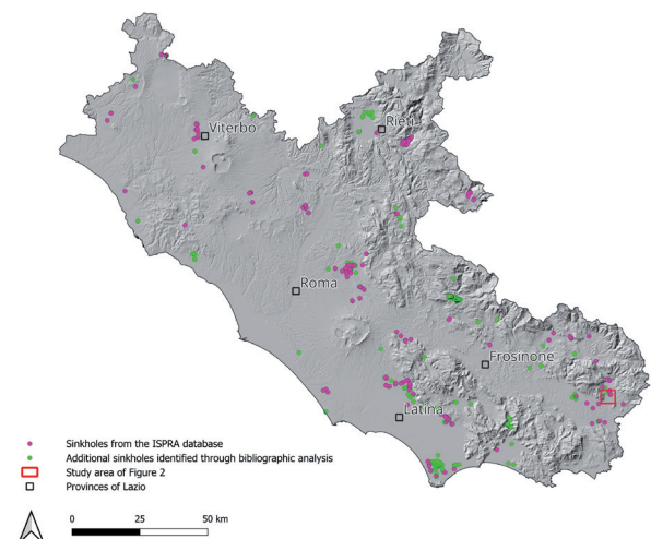
Fig. 3 - Distribution of sinkholes inventoried by the ISPRA Database and bibliographic analysis
