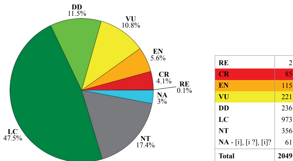
Fig. 6 – Percentages of the IUCN categories of risk among the 2049 listed Italian saproxylic beetle species.
