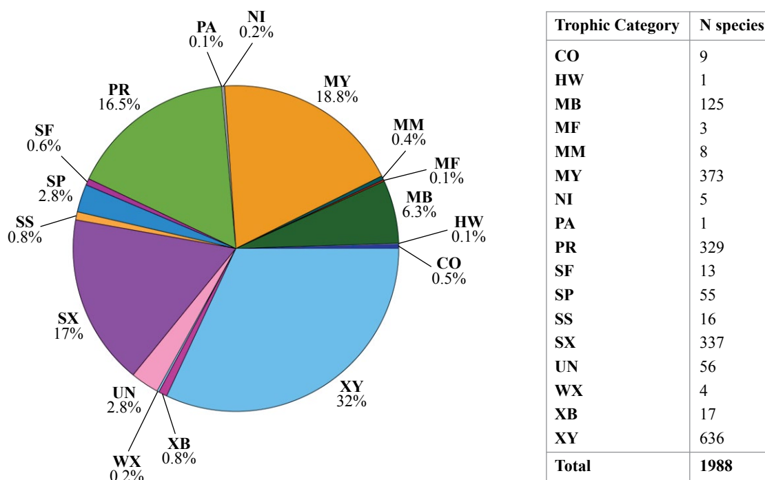
Fig. 9 – Percentages of the 1988 Italian assessed saproxylic beetles (excluding NA, i.e. all the 61 introduced species) included in each of the 18 Trophic Categories listed in Table 3 (the AR Trophic Category, only including two alien species occasionally present in natural habitats, is not listed here).
