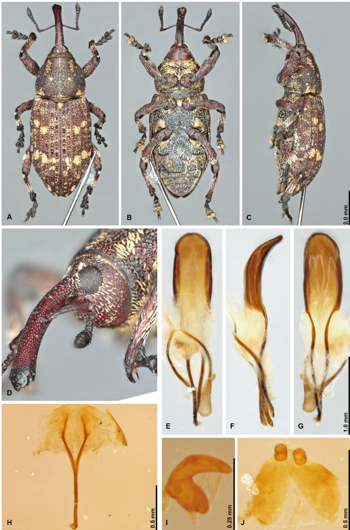
Fig. S19. Habitus and genitalia of Pissodes pini . A-C: habitus dorsal, ventral and lateral of female, D: dorso-lateral view on head and rostrum, E-G: penis in dorsal, lateral and ventral view, H: female sternite VIII, I: spermatheca, J: gonocoxites, © Christoph Germann.
