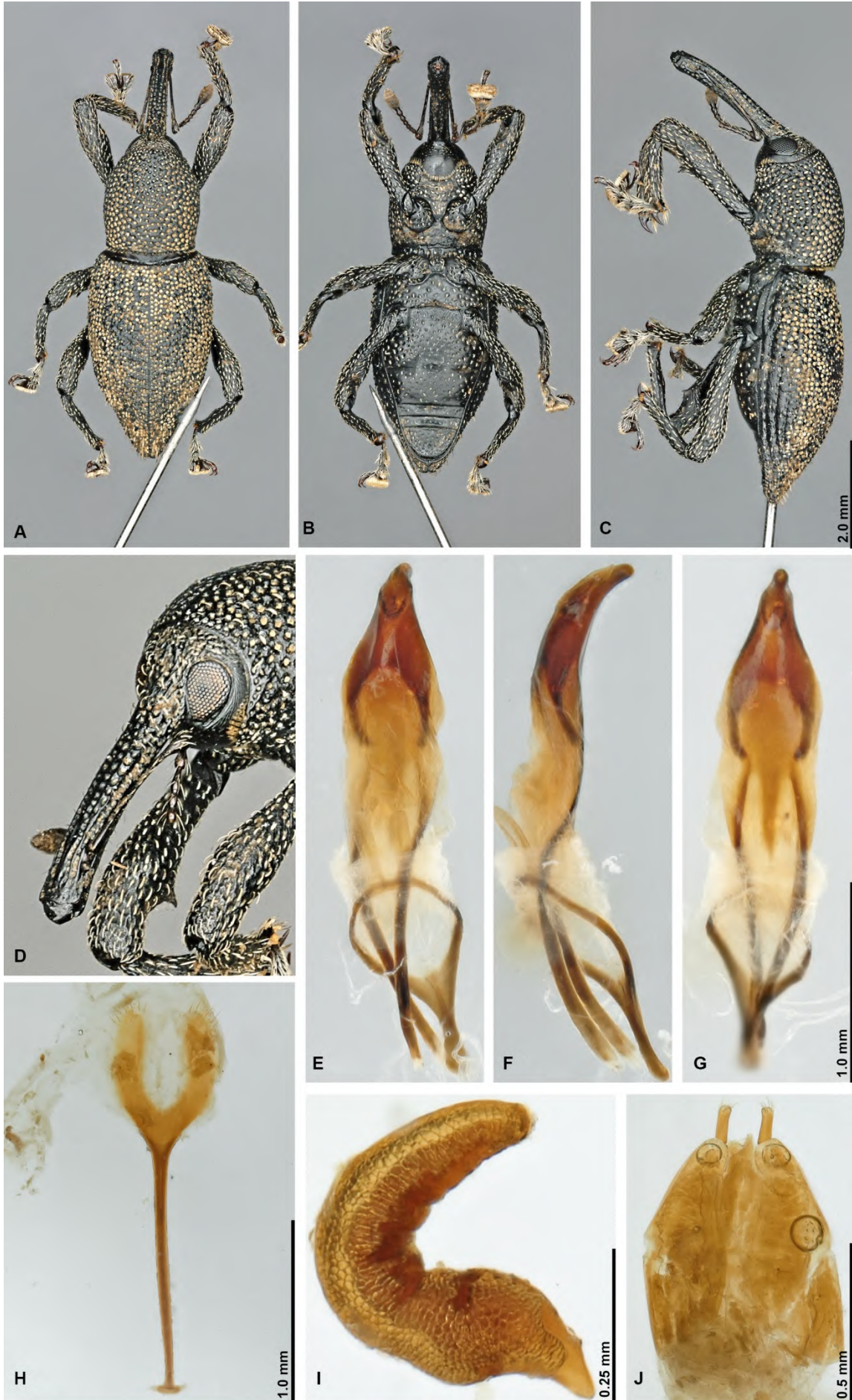
Fig. S18. Habitus and genitalia of Pinacopus intermedius . A-C: habitus dorsal, ventral and lateral of female, D: dorso-lateral view on head and rostrum, E-G: penis in dorsal, lateral and ventral view, H: female sternite VIII, I: spermatheca, J: gonocoxites, © Christoph Germann.
