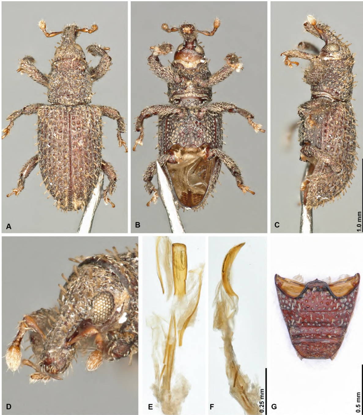
Fig. S16. Habitus and genitalia of a species in a genus near Pseudohylobius . A-C: habitus dorsal, ventral and lateral of male, D: dorso-lateral view on head and rostrum, E-F: penis in ventral and lateral view, G: ventrites, © Christoph Germann.
