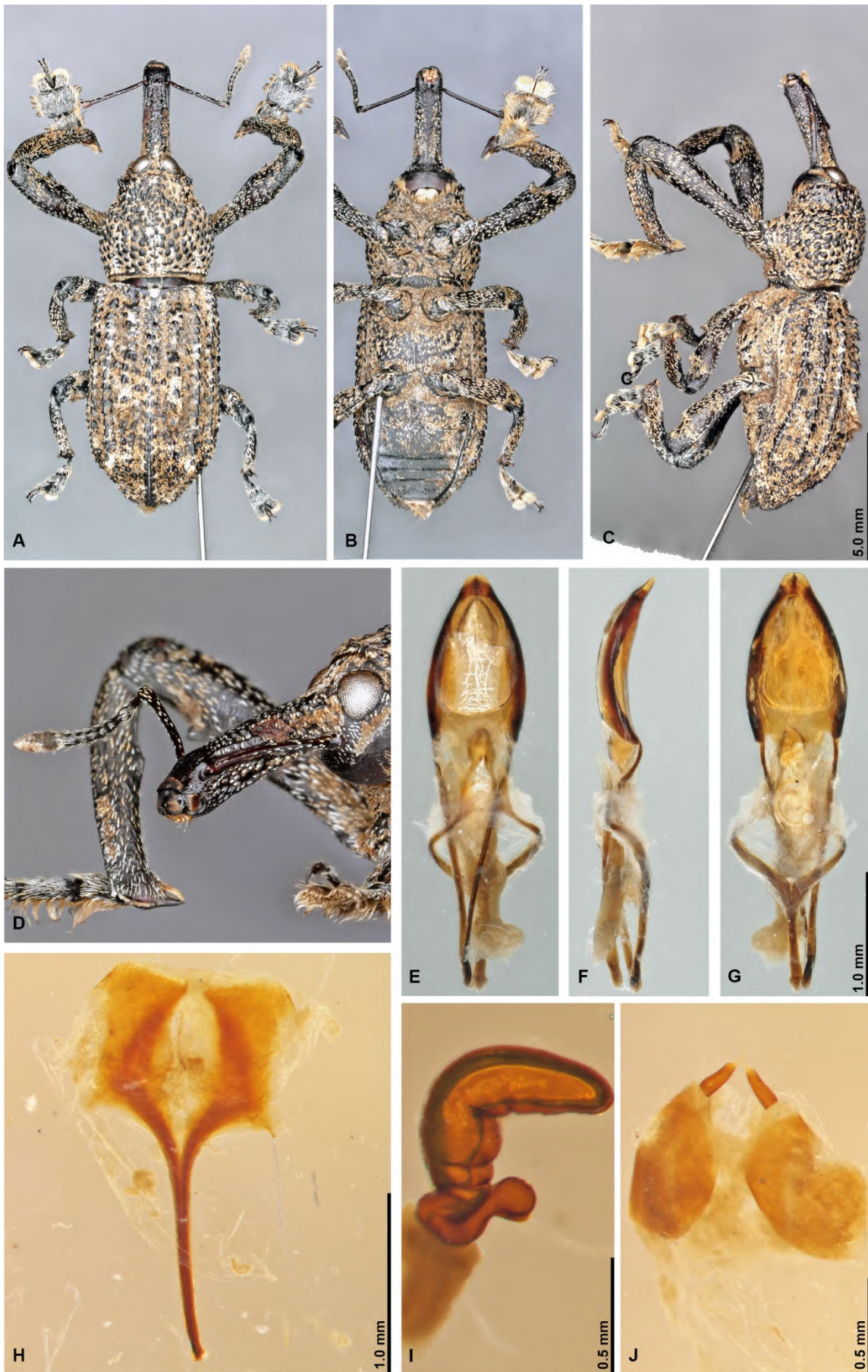
Fig. S17. Habitus and genitalia of Orthorhinus sp. A-C: habitus dorsal, ventral and lateral of male, D: dorso-lateral view on head and rostrum, E-G: penis in dorsal, lateral and ventral view, H: female sternite VIII, I: spermatheca, J: gonocoxites, © Christoph Germann.
