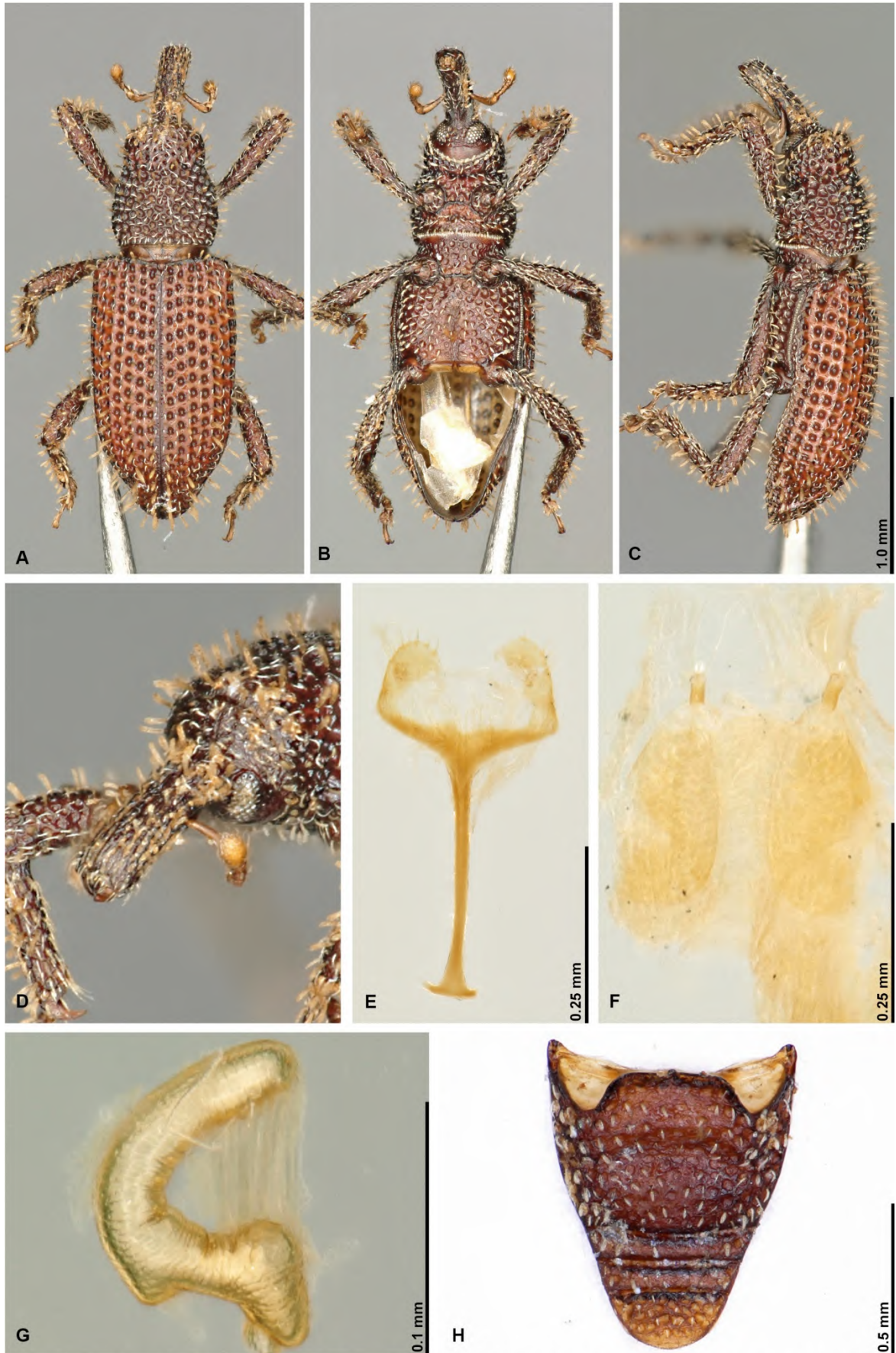
Fig. S21. Habitus and genitalia of Seticotasteromimus sp. A-C: habitus dorsal, ventral and lateral of female, D: dorso-lateral view on head and rostrum, E: female sternite VIII, F: gonocoxites, G: spermatheca, H: ventrites, © Christoph Germann.
