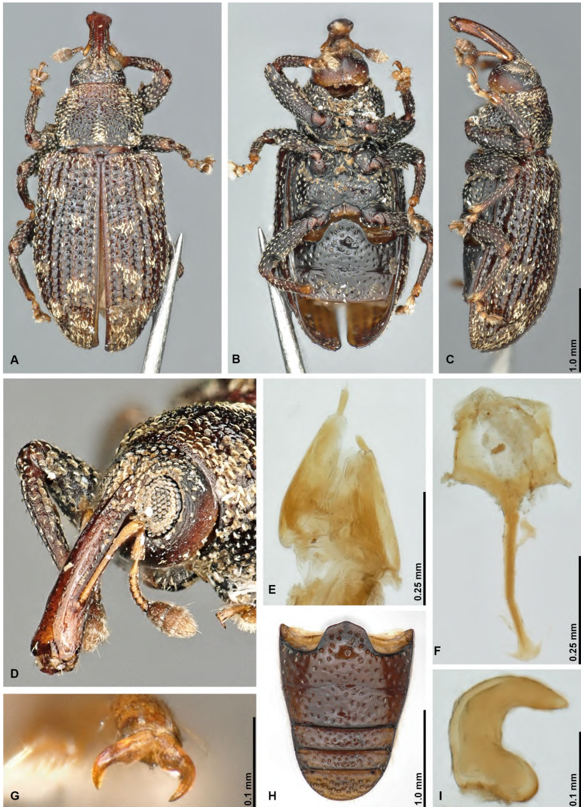
Fig. S9. Habitus and genitalia of Dorytomorpha tonsa . A-C: habitus dorsal, ventral and lateral of female, D: dorso-lateral view on head and rostrum, E: gonocoxites, F: sternite VIII, G: claws, H: ventrites, I: spermatheca, © Christoph Germann.
