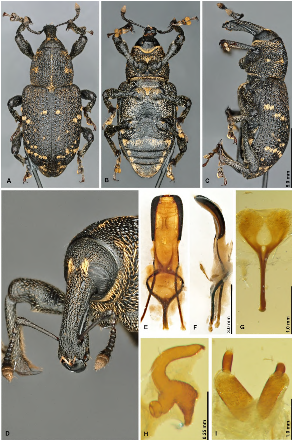
Fig. S12. Habitus and genitalia of Hylobius abietis . A-C: habitus dorsal, ventral and lateral of male, D: dorso-lateral view on head and rostrum, E-F: penis in dorsal and lateral view, G: sternite VIII, H: spermatheca, I: gonocoxites, © Christoph Germann.
