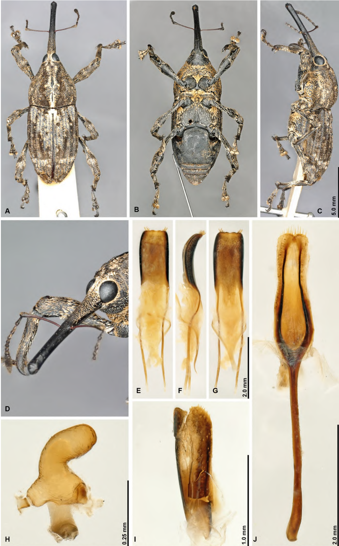
Fig. S13. Habitus and genitalia of Ilacuris laticollis . A-C: habitus dorsal, ventral and lateral of male, D: dorso-lateral view on head and rostrum, E-G: penis in dorsal, lateral and ventral view, H: spermatheca, I: gonocoxites, J: female sternite VIII, © Christoph Germann.
