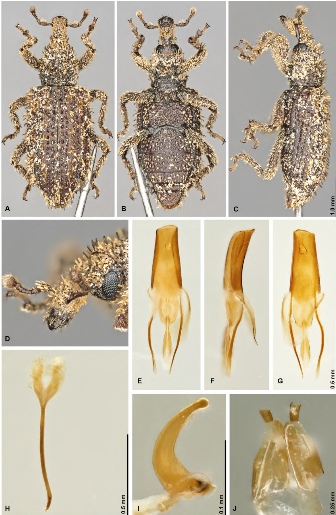
Fig. S20. Habitus and genitalia of Pseudohylobius setosus . A-C: habitus dorsal, ventral and lateral of female, D: dorso-lateral view on head and rostrum, E-G: penis in dorsal, lateral and ventral view, H: female sternite VIII, I: spermatheca, J: gonocoxites, © Christoph Germann.
