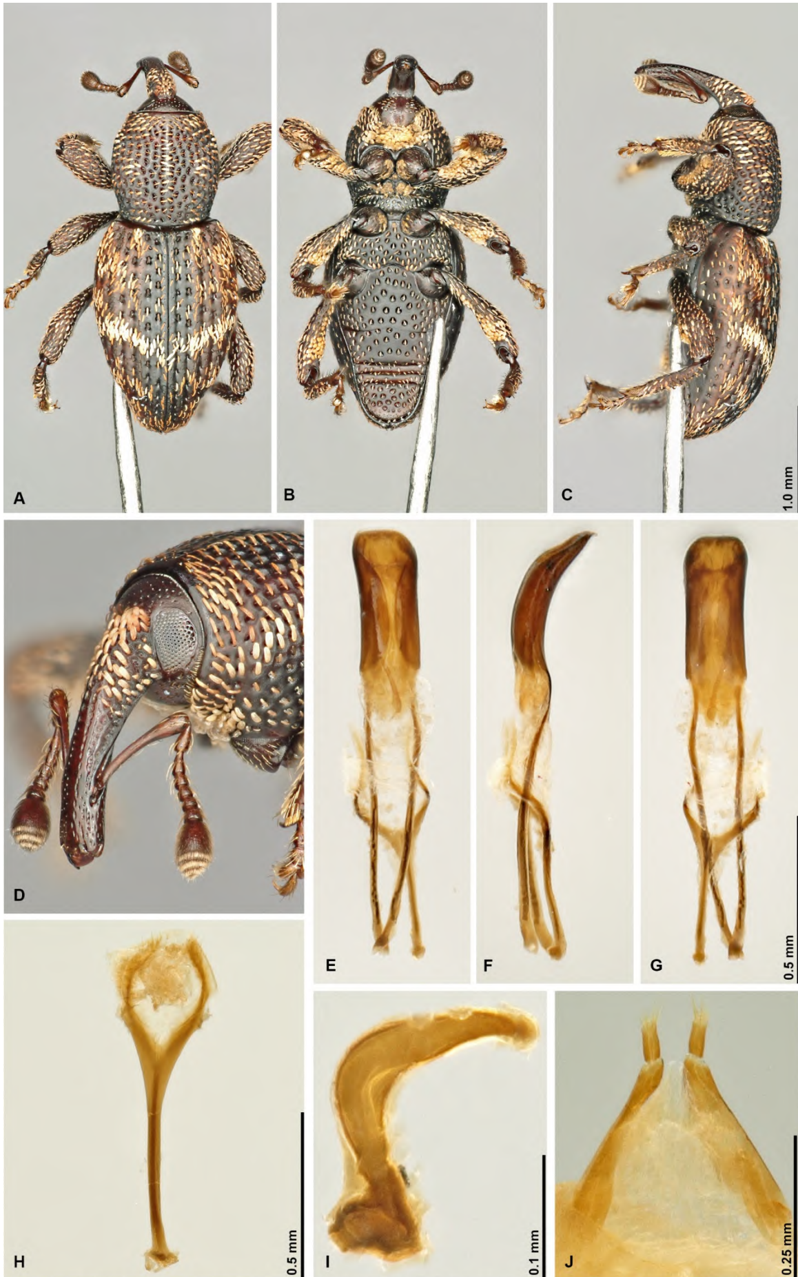
Fig. S11. Habitus and genitalia of Himalanchonus sp. A-C: habitus dorsal, ventral and lateral of male, D: dorso-lateral view on head and rostrum, E-G: penis in dorsal, lateral and ventral view, H: female sternite VIII, I: spermatheca, J: gonocoxites, © Christoph Germann.
