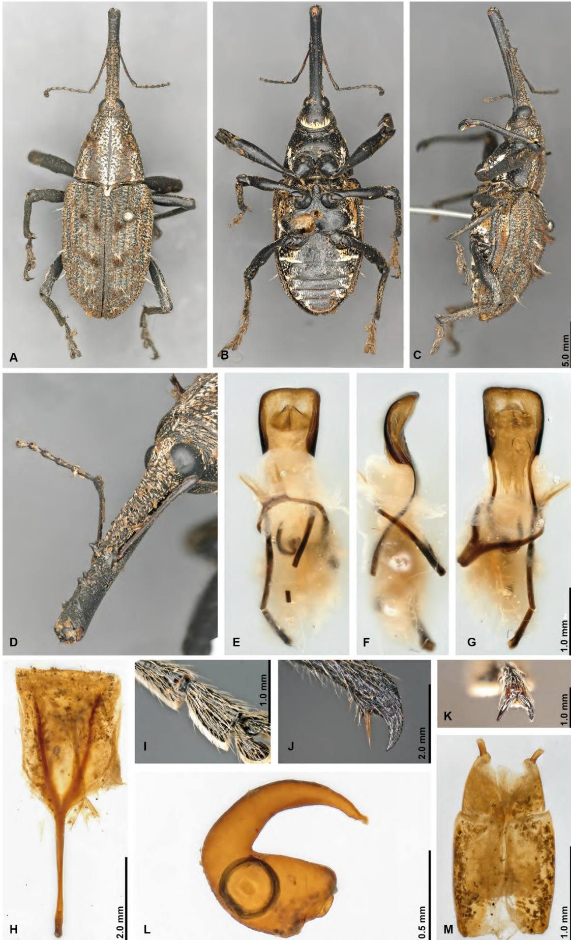
Fig. S10. Habitus and genitalia of Eurhamphus fasciculatus . A-C: habitus dorsal, ventral and lateral of male, D: dorso-lateral view on head and rostrum, E-G: penis in dorsal, lateral and ventral view, H: female sternite VIII, I: tarsus (flattened second tarsomere), J: premucro and uncus on apex of left protibia, K: claws, L: spermatheca, M: gonocoxites, © Christoph Germann.
