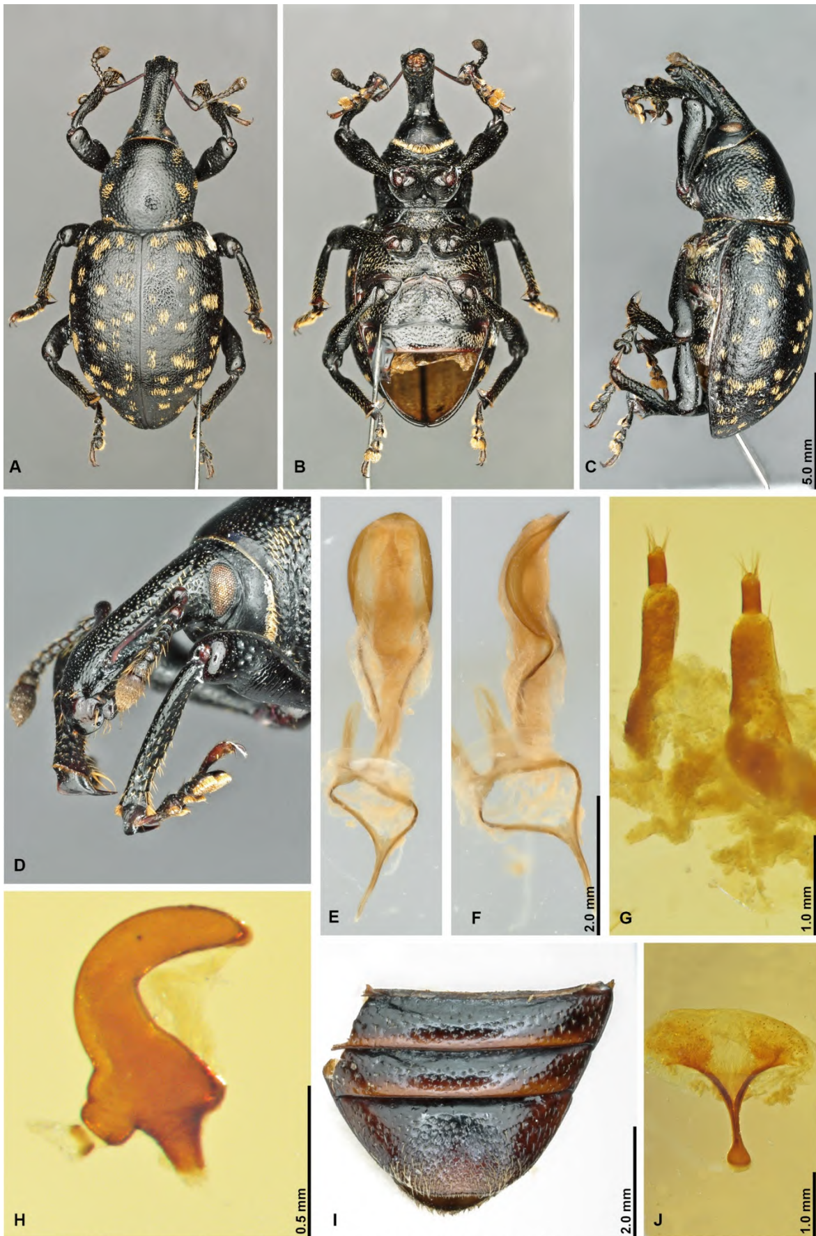
Fig. S15. Habitus and genitalia of Liparus germanus . A-C: habitus dorsal, ventral and lateral of male, D: dorso-lateral view on head and rostrum, E-F: penis in dorsal and lateral view, G: gonocoxites, H: spermatheca, I: last three ventrites, J: female sternite VIII, © Christoph Germann.
