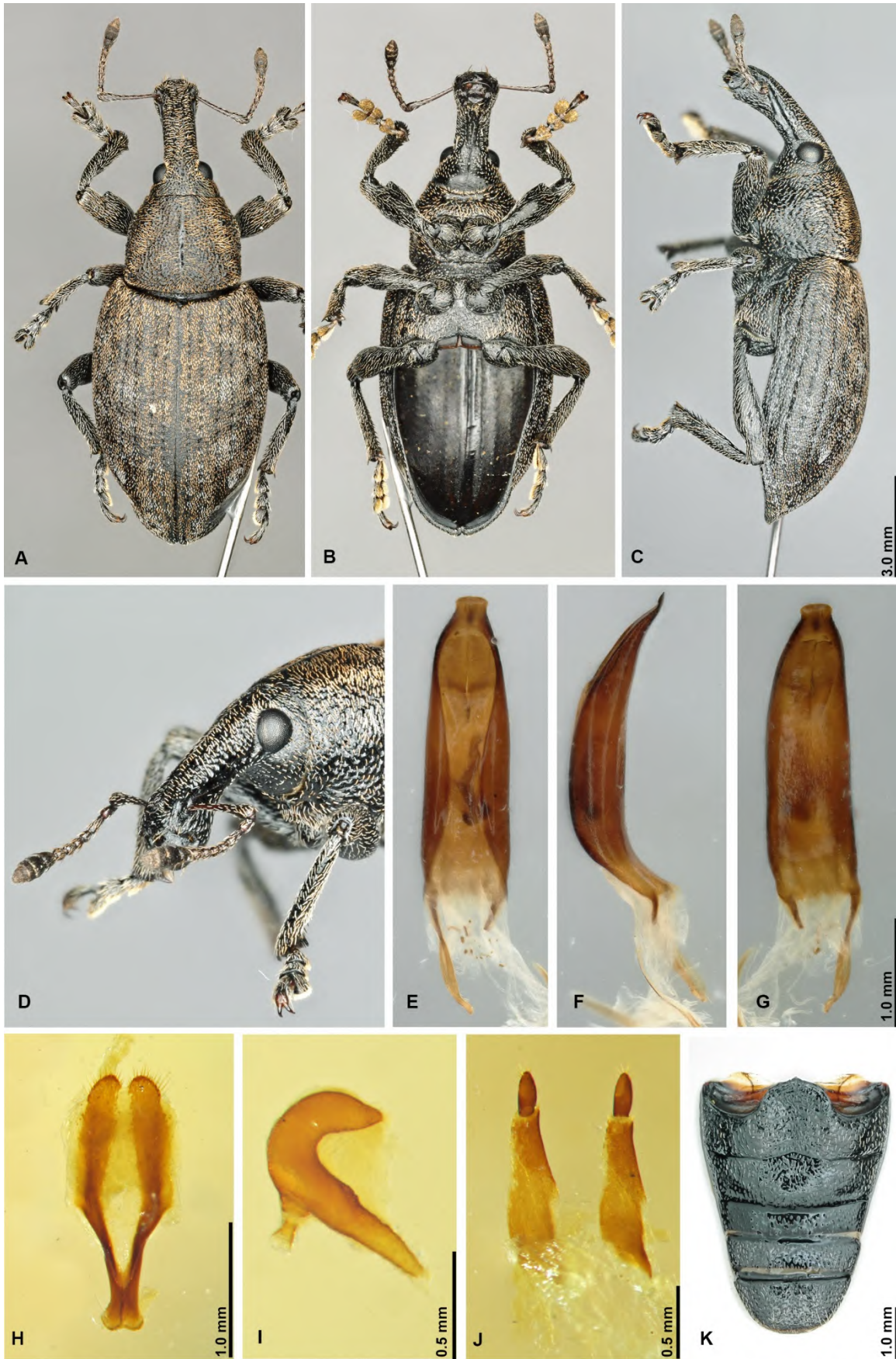
Fig. S14. Habitus and genitalia of Lepyrus capucinus . A-C: habitus dorsal, ventral and lateral of male, D: dorso-lateral view on head and rostrum, E-G: penis in dorsal, lateral and ventral view, H: female sternite VIII, I: spermatheca, J: gonocoxites, K: ventrites, © Christoph Germann.
