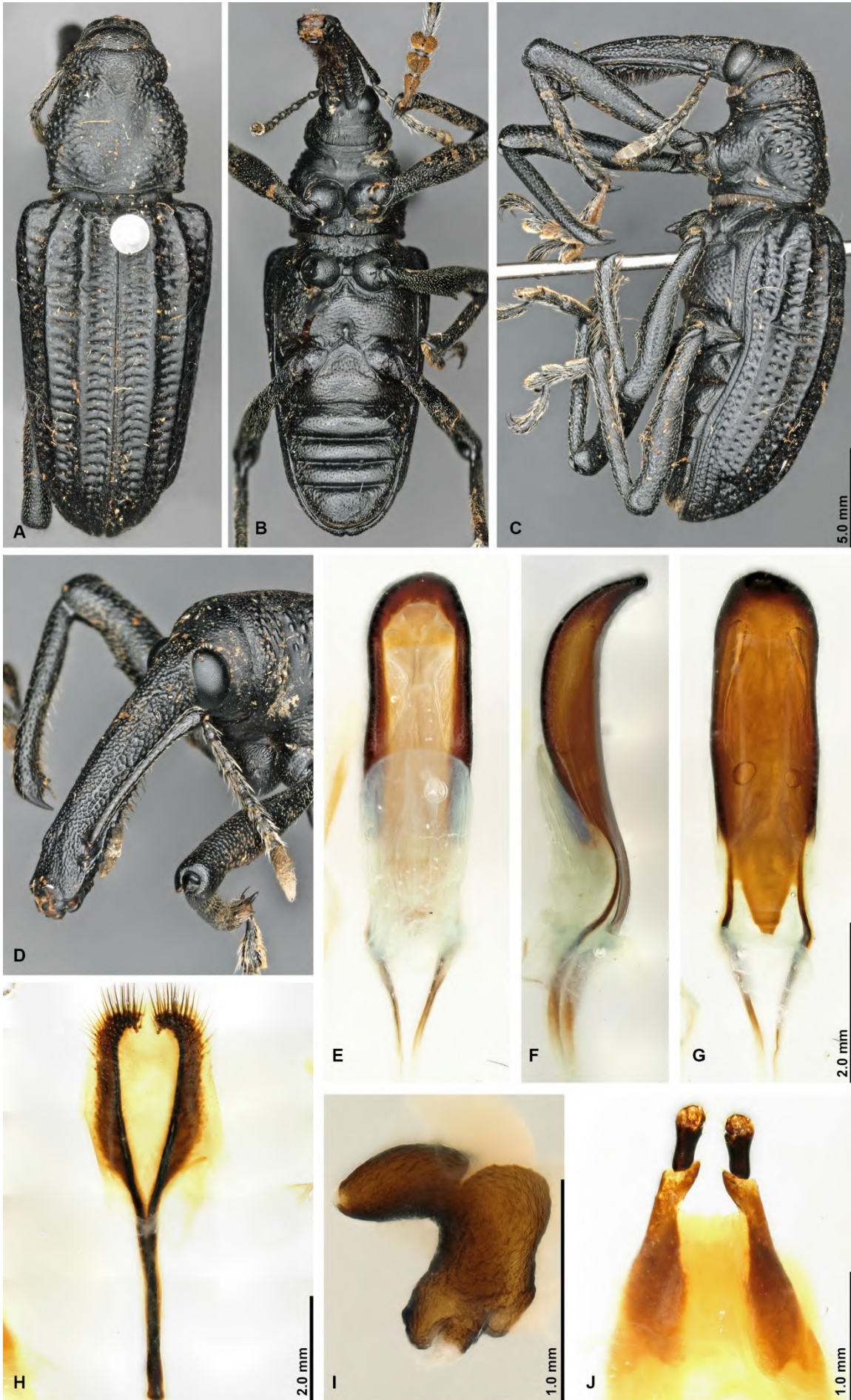
Fig. S22. Habitus and genitalia of Vanapa oberthuri . A-C: habitus dorsal, ventral and lateral of female, D: dorso-lateral view on head and rostrum, E-G: penis in dorsal, lateral and ventral view, H: female sternite VIII, I: spermatheca, J: gonocoxites, © Christoph Germann.
