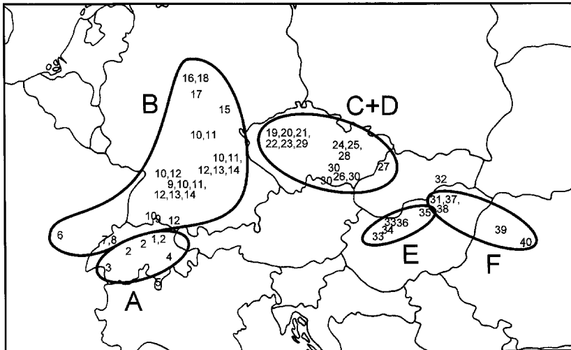
Fig. 4 - Geographical differentiation of the Tilia -dominated calcicolous forests in Central Europe. Capital letters refer to the groups discussed in the text; numbers denote the data sources listed in Appendix 2.
