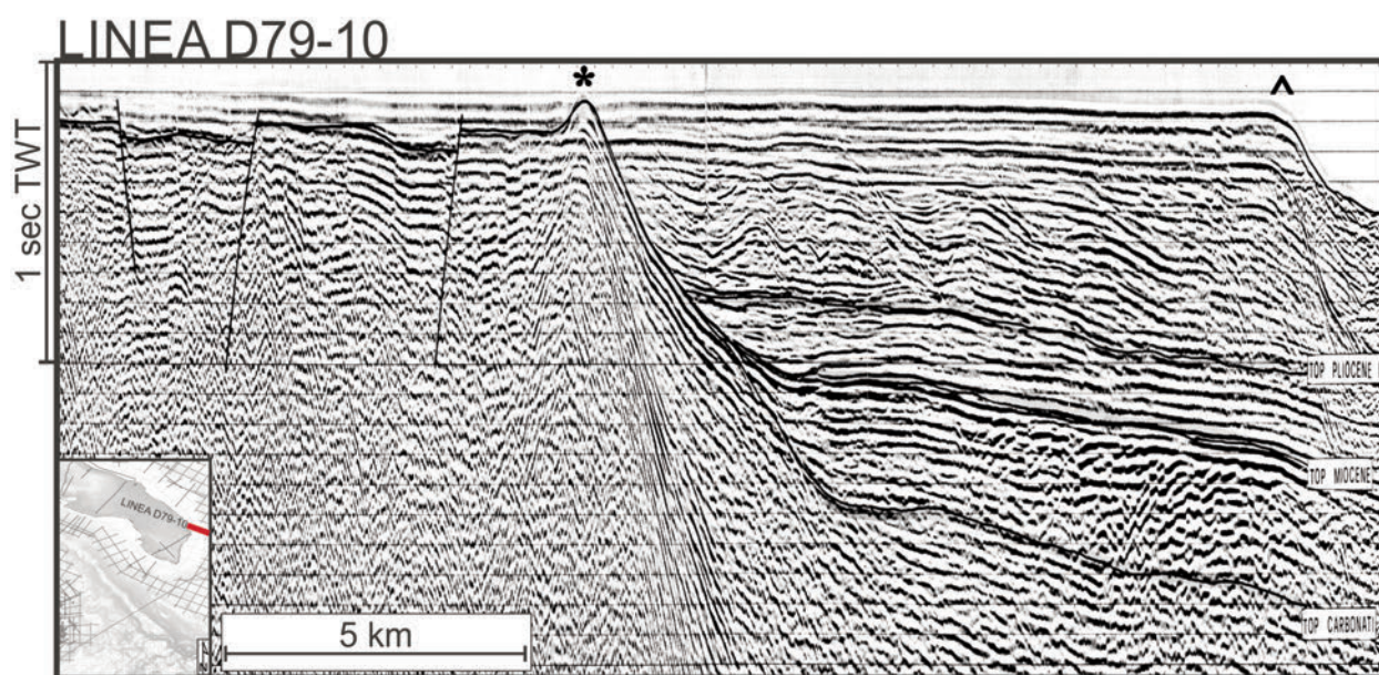
Fig. 1 - Seismic line (with the original interpretation by AGIP) showing the Mesozoic platform margin (*) and the Pleistocene shelf margin (^). Location of the line in the inset.
