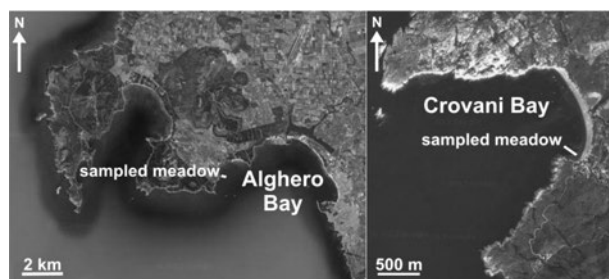
Fig. 1 - Alghero Bay (Sardinia, Italy) and Crovani Bay (Corsica, France): location maps (images modified from Google Maps).
