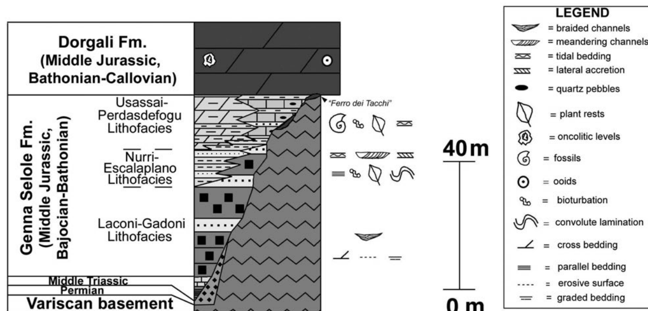
Fig. 2 - Stratigraphic column and general framing of the FGS in eastern Sardinia.
