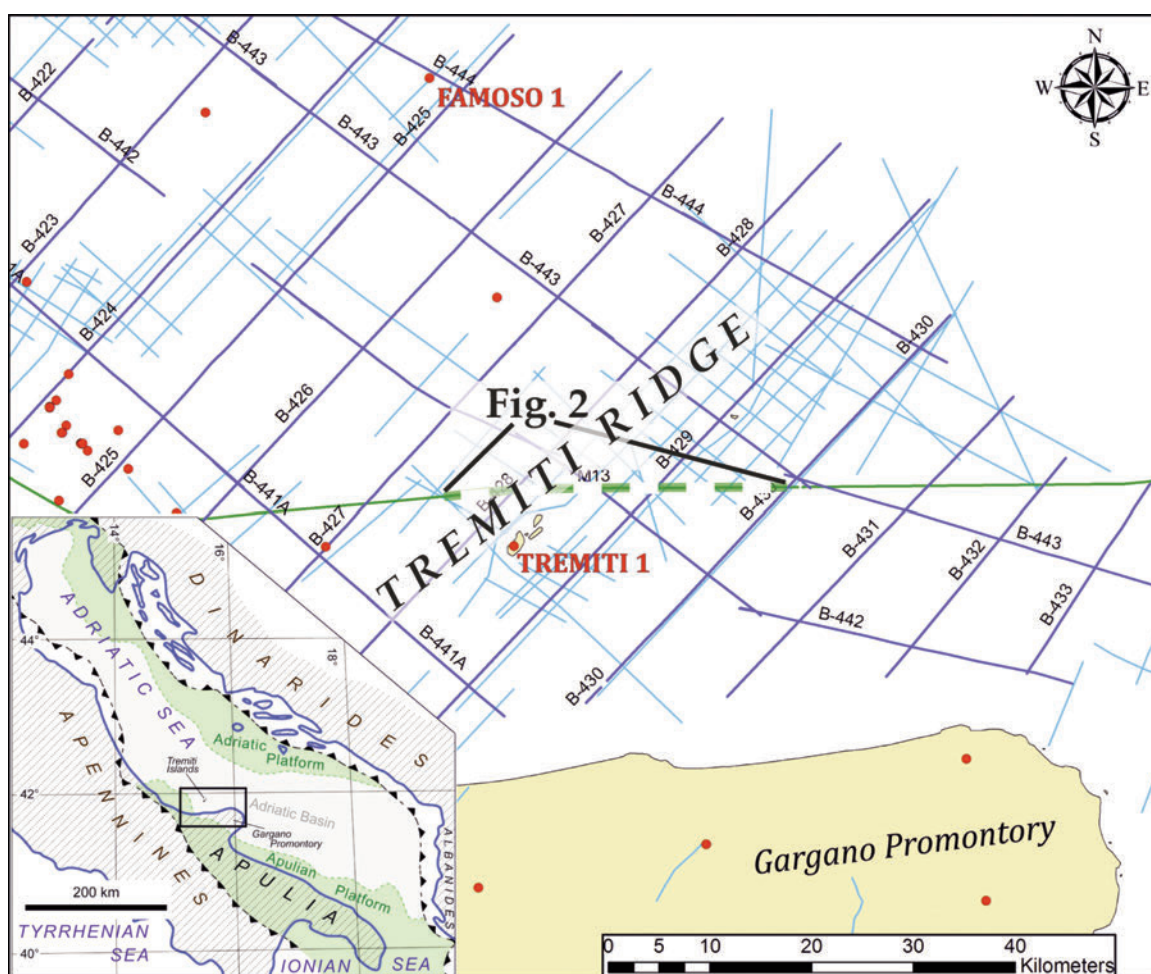
Fig. 1 - Seismic lines and wells coming from both ViDEPI and CROP Projects. The Tremiti ridge is roughly NE-SW elongated.
