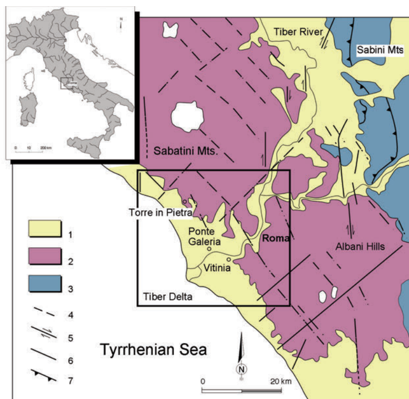
Fig. 1 - Geological sketch of the Tyrrhenian margin, central Italy. 1) Messinian to Holocene sedimentary deposits; 2) Plio-Pleistocene lavas and volcanoclastic deposits; 3) Meso-Cenozoic sedimentary deposits; 4) main buried faults; 5) strike-slip faults; 6) normal faults; 7) major thrusts. The black square indicates the study area.
