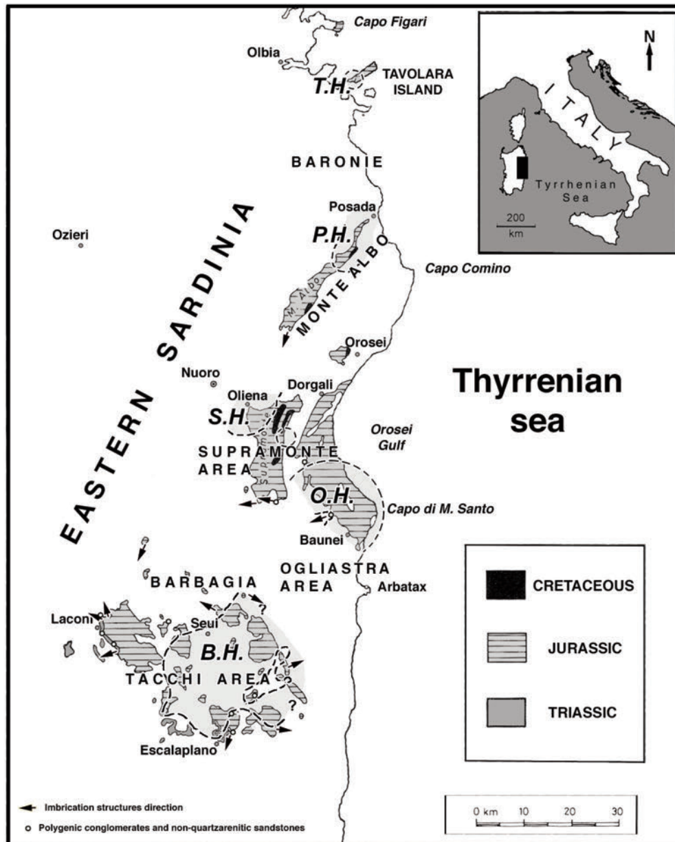
Fig. 1 - Localization of the investigated area. Legend: B.H.: Barbagia High; O.H.: Ogliastra High; S.H.: Supramonte High; P.H.: Posada High; T.H.: Tavolara High.
