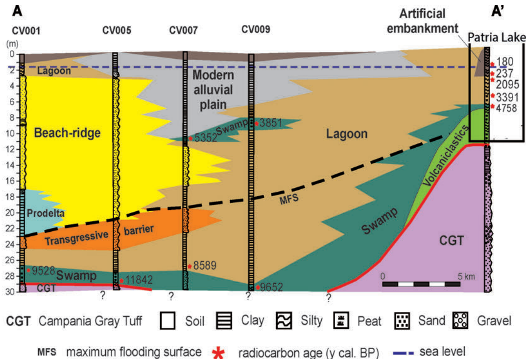
Fig. 3 - Facies architecture of Volturno plain in stratigraphic cross-sections sub-parallel to the present-day shoreline (see Fig. 1 for section trace). Box indicate the present-day position of Patria Lake.
