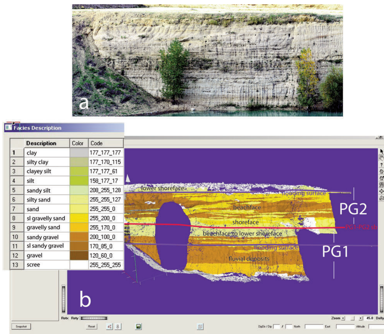
Fig. 3 - Dip-section photo panel of the Tiberi quarry (a) exposing the PG1 and PG2 sequences and Geco interpretation window (b) showing the distribution of grain-size classes and depositional environments.
