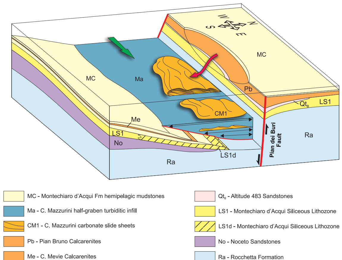
Fig. 22 - Three-dimensional reconstruction of the geometry and architecture of C. Mazzurini Half-graben fill, with indication of axial and lateral transport directions.
