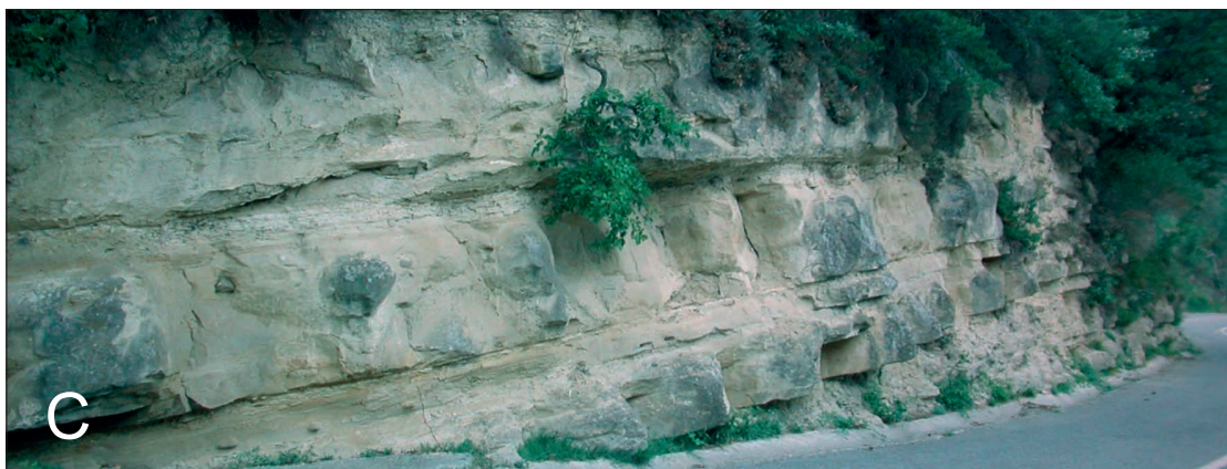
Fig. 23 - Facies samples in the Piantivello unit. a) Bric Arborella section (cf. Fig. 2 and Pl. VIc). b) C. Poggi II section (cf. Fig. 2 and Pl. VIb). c) Thick-bedded sandstone-mudstone couplets in the basal part of C. Poggi II section.
