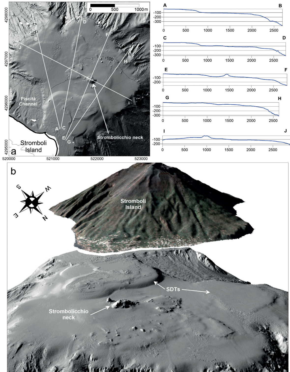
Fig. 3 - a) Shaded relief map of the NE shelf, with the trace of the bathymetric profiles shown on the left. b) 3-D view of the NE shelf; SDT: submarine depositional terrace.
