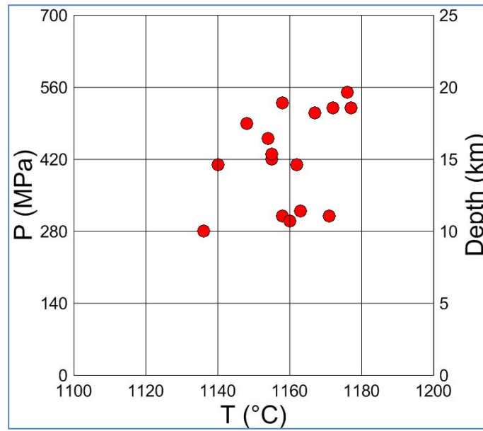
Fig. 1. A plot showing the calculated temperatures for the mafic end member of the NGP using the clinopyroxene-only thermometer (Eq. 32d) and barometer (Eq. 32a) of Putirka et al. (2008b).
