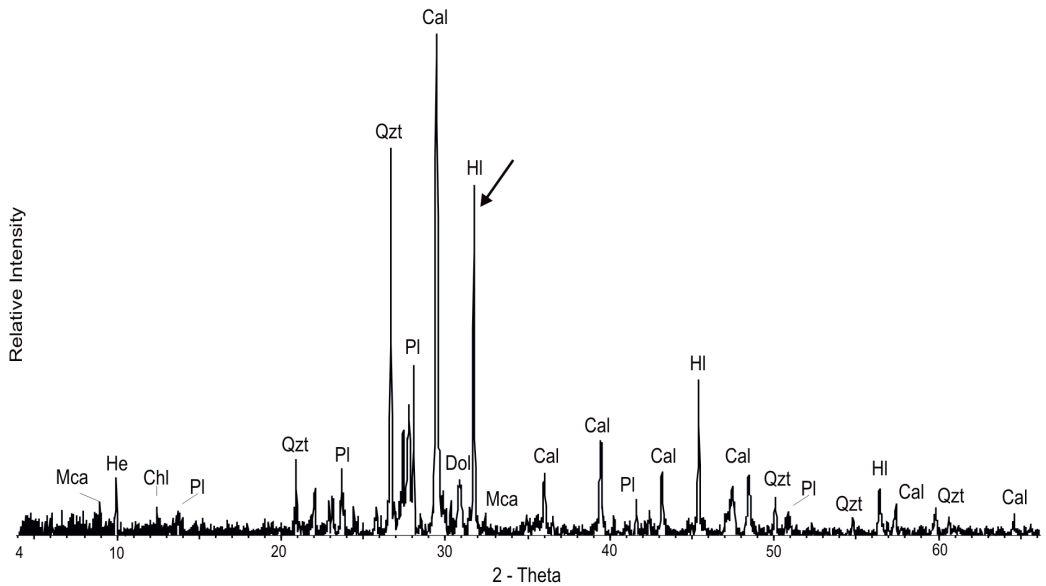
Figure 7. X-ray diffraction patterns of sample KM21 with identification of the principal mineralogical phases (Cal = Calcite; Chl = Chlorite; Dol = Dolomite; He = Heulandite; HI = Halite; Mca = Mica; Pl = Plagioclase; Qzt = Quartz).
