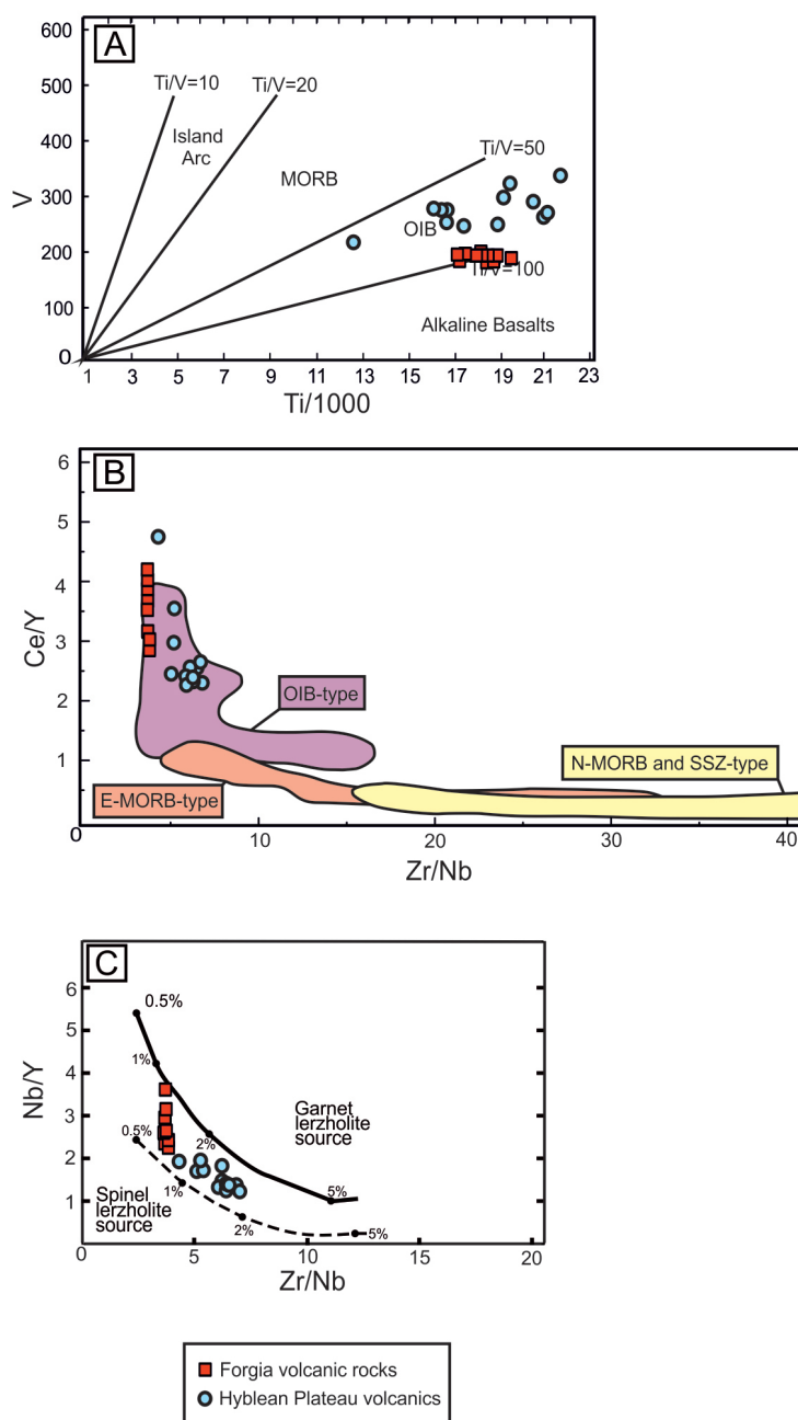
Figure 8. Discrimination diagrams of the Forgia volcanics: A) V vs Ti plot from Shervais (1982); B) Zr/Nb vs Ce/Y diagram after Göncüoğlu et al., 2010 - Fields for the OIB-, E-MORB, N-MORB, and SSZ-type basaltic rocks are taken from Maheo et al. (2004), and Aldanmaz et al. (2008). C) Zr/Nb vs Nb/Y diagram (after Harangi, 2001). For comparison, data from Hyblean Plateau (after Avanzinelli et al., 2012) are plotted.
