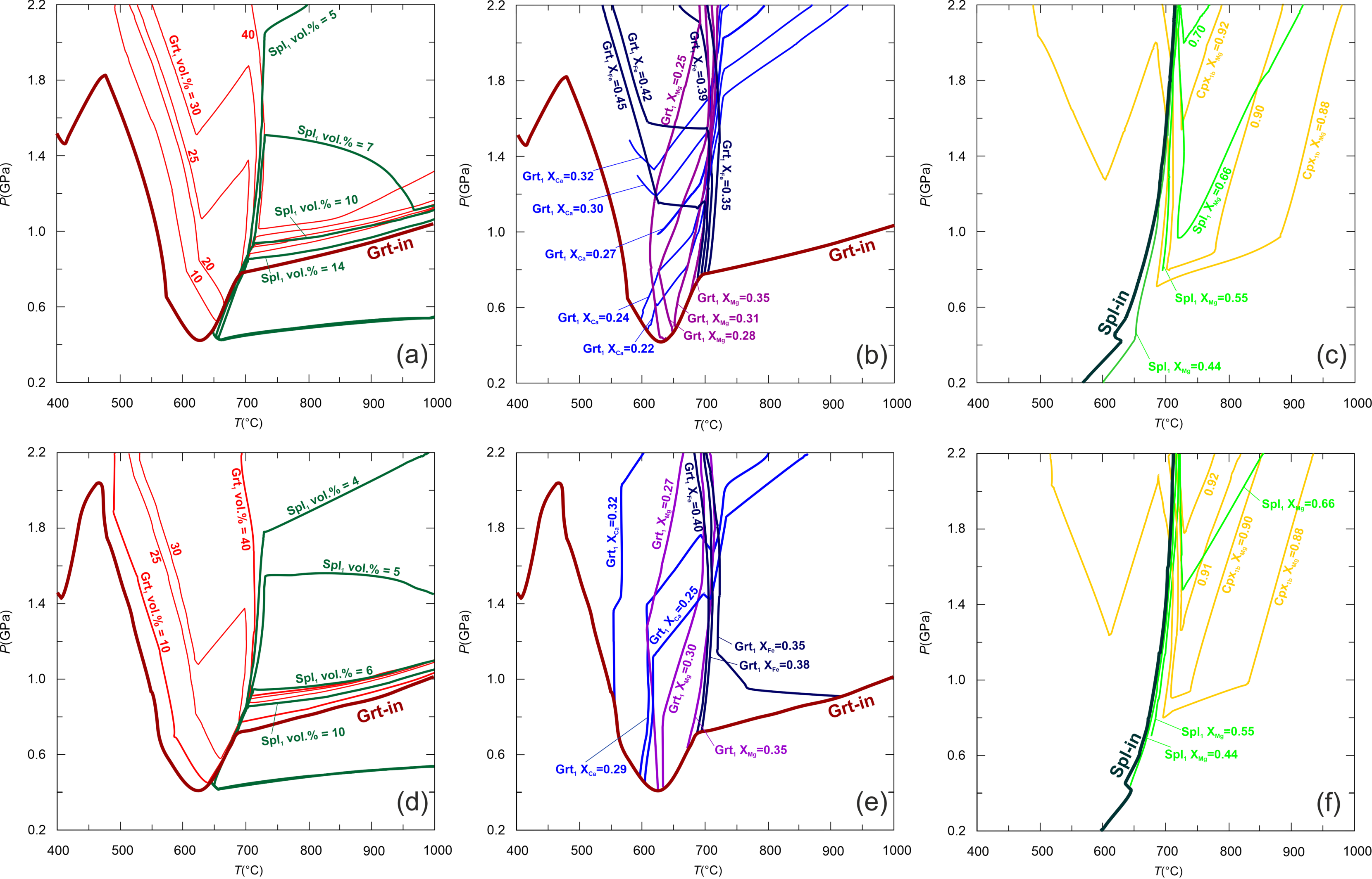
Figure S1. Mineral isomodes and isopleths for samples MNX and MNY. Sample MNX: (a) garnet and spinel isomodes (vol.%); (b) X_{Ca} , X_{Mg} and X_{Fe} compositional isopleths for garnet; (c) X_{Mg} compositional isopleths for Spl 1 and Cpx 1b . Sample MNY: (d) garnet and spinel isomodes (vol.%); (e) X_{Ca} , X_{Mg} and X_{Fe} compositional isopleths for garnet; (f) X_{Mg} compositional isopleths for Spl 1 and Cpx 1b .
