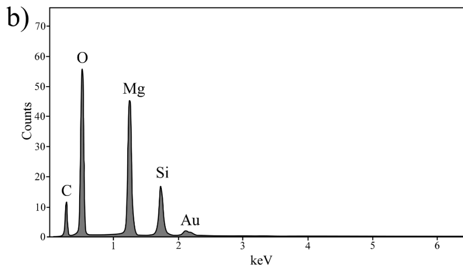
Figure S1. Representative SEM images (a) and EDX spectrum (b) of lizardite particle found in the sample.
