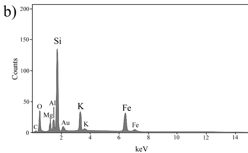
Figure S3. Representative SEM images (a) and EDX spectrum (b) of phlogopite particle found in the sample.
