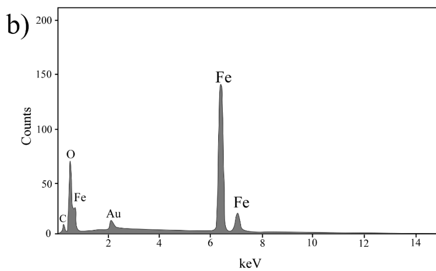
Figure S4. Representative SEM images (a) and EDX spectrum (b) of magnetite particle found in the sample.
