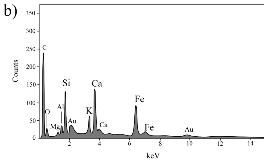
Figure S5. Representative SEM images (a) and EDX spectrum (b) of allotriomorphs fragments of Si-, Al- and Ca- bearing phase(s) found in the sample.
