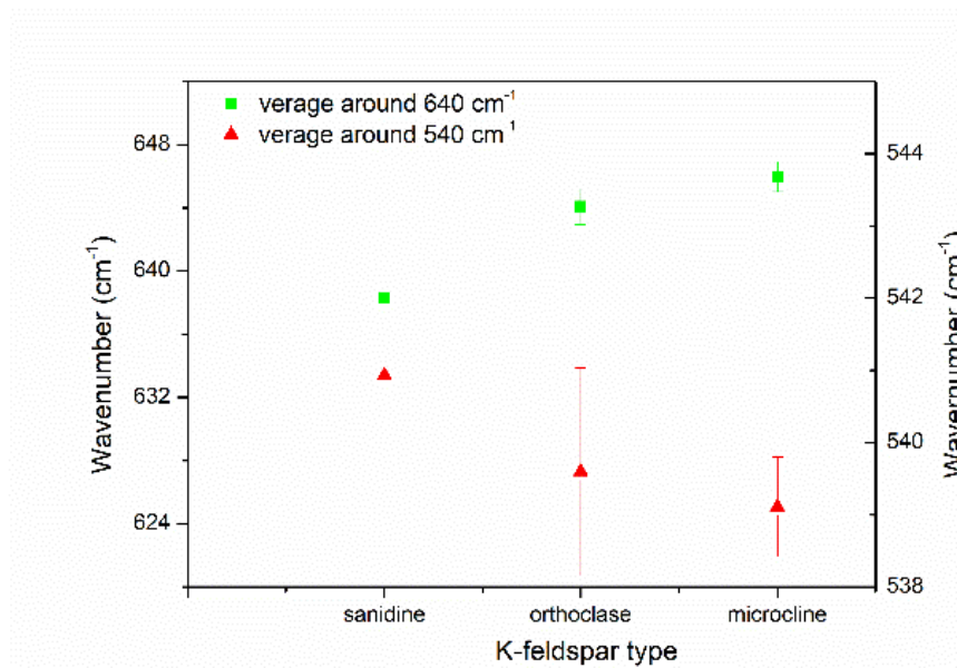
Figure S1. Wavenumber shift around 540 cm -1 and 640 cm -1 with different K-feldspar types. The wavenumber values of five orthoclase samples and five microcline samples were averaged respectively. The vertical bars represent errors. If no bar is given, then the error is contained within the area of the symbol.
