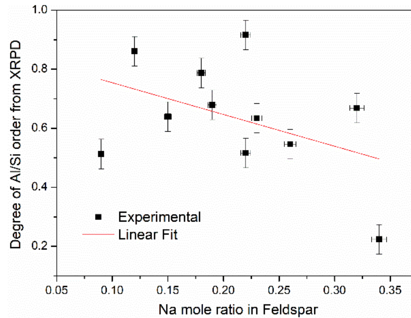
Figure S2. Plot of degree of Al/Si order from XRPD against Na mole ratio in feldspar (Pearson's R=-0.44 , P=0.18 ). The vertical bars represent errors. If no bar is given, then the error is contained within the area of the symbol (the relative errors of Na mole ratio were estimated to be about 2% in terms of XRF measurement accuracy).
