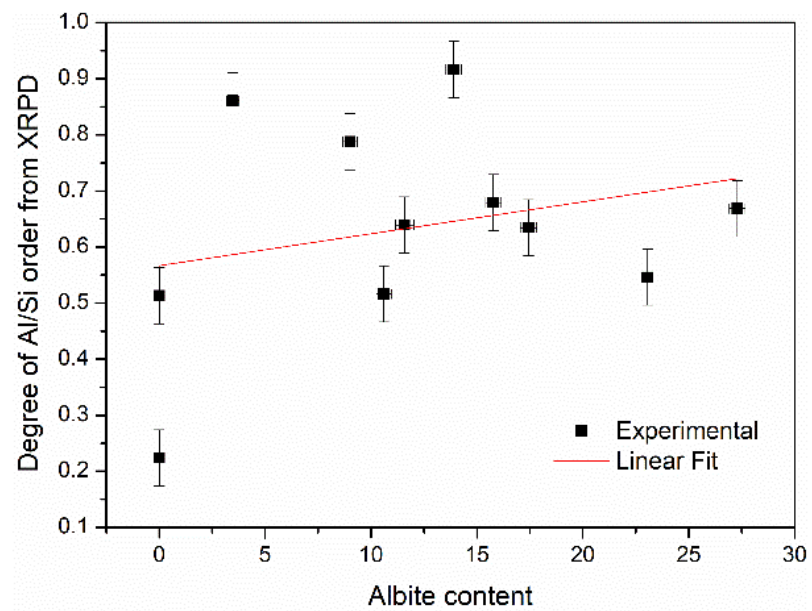
Figure S3. Plot of degree of Al/Si order from XRPD against albite content in feldspar (Pearson's R=0.26 , P=0.43 ). The vertical bars represent errors. If no bar is given, then the error is contained within the area of the symbol.
