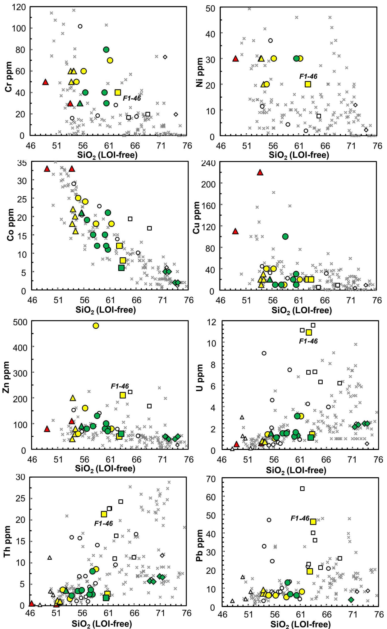
Figure S1. Additional trace elements vs \text{SiO}_2 binary variation diagrams for Tafresh area rock samples (this work and available literature) and for selected literature data for the UDMA rocks with “orogenic” affinity. A highlight on sample F1-46 is provided where its composition is significantly deviating from that of the other evolved samples. Symbols and sources of bibliographic data as in Figure 4.
