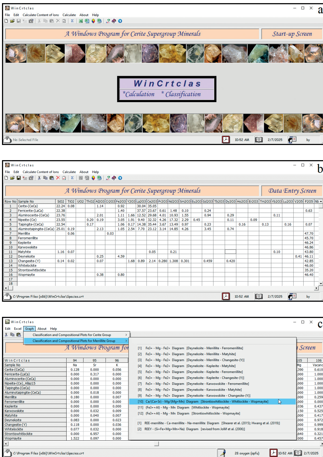
Figure 1. a) A screenshot of the WinCrtclas Start-up window with various pull-down menus and equivalent shortcuts. b) A screenshot of the WinCrtclas Data Entry window with a total of 41 analytes (wt%). c) A screenshot of the WinCrtclas Calculation Screen with plot options from the pull-down menu of the Graph .
